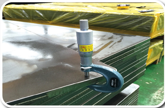
Thickness : +/- 0.2mm
